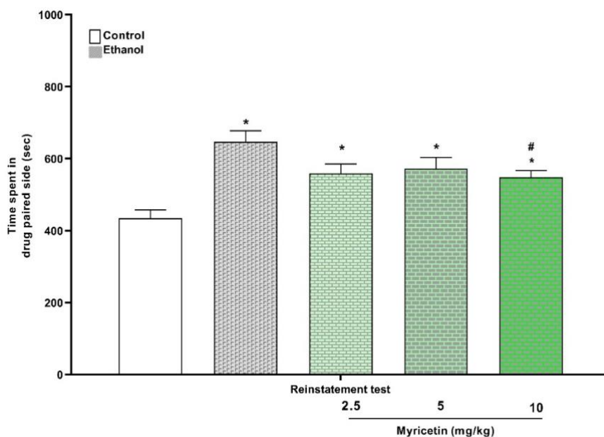
Figure 3. Effects of myricetin (2.5, 5 and 10 mg/kg) on the reinstatement of ethanol CPP caused by ethanol (0.4 g/kg). Results are shown as mean ( \pm SEM) values ( n=6-8 ). * p < 0.01 versus the saline group; # p < 0.05 versus the ethanol group.
