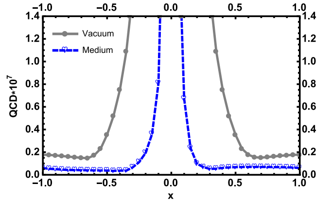
FIG. 2. Variation of QCD side as a function of x obtained using the structure \not{x} at \Xi_{cc} channel.
