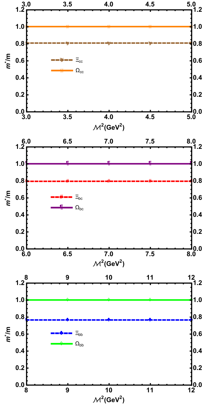
FIG. 4. The in-medium mass to vacuum mass ratio m^*/m with respect to Borel mass \mathcal{M}^2 for the spin-1/2 doubly heavy \Xi_{QQ'} and \Omega_{QQ'} baryons at average value of continuum threshold and at saturation nuclear matter density.
