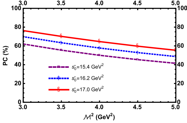
FIG. 3. PC with respect to \mathcal{M}^2 for the \Xi_{cc} channel and the structure \bar{p} at \rho = \rho_{sat} and x = 0.85 .
