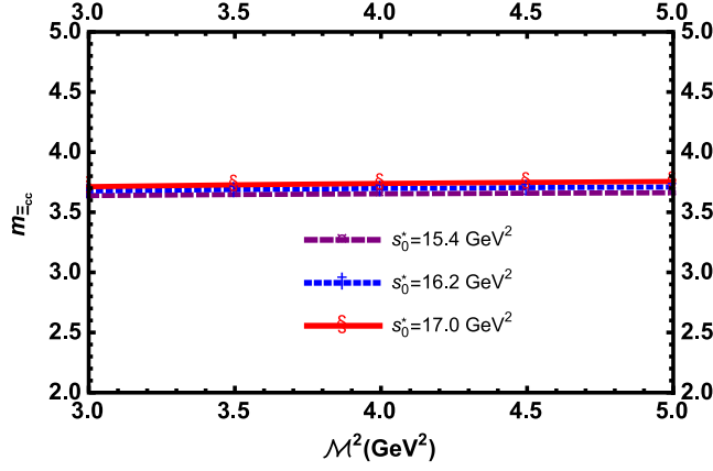
FIG. 1. m_{\Xi_{cc}} as a function of \mathcal{M}^2 at three different values of in-medium continuum threshold.
