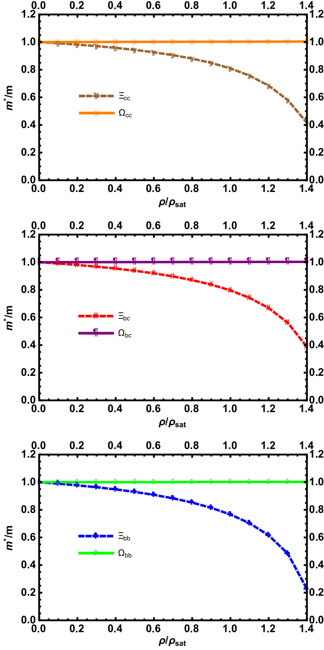
FIG. 5. The in-medium mass to vacuum mass ratio m^*/m of the doubly heavy \Xi_{QQ'} and \Omega_{QQ'} baryons with respect to \rho/\rho_{\text{sat}} at average values of continuum threshold and Borel mass parameter.
