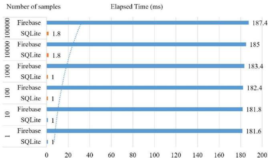
Figure 3. The experimental result of querying different numbers of data from SQLite and Firebase
