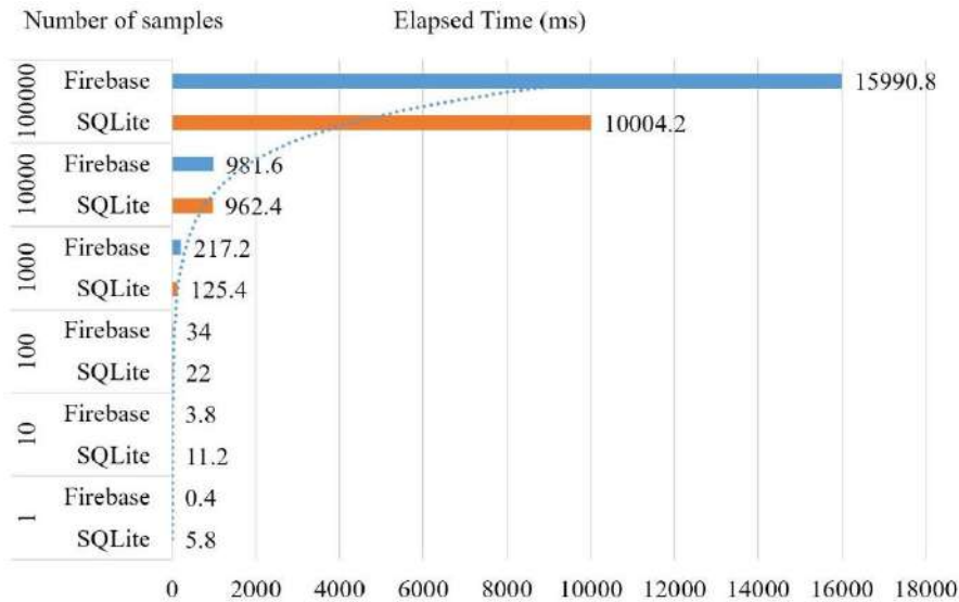
Figure 2. The experimental result of inserting different numbers of data into SQLite and Firebase
