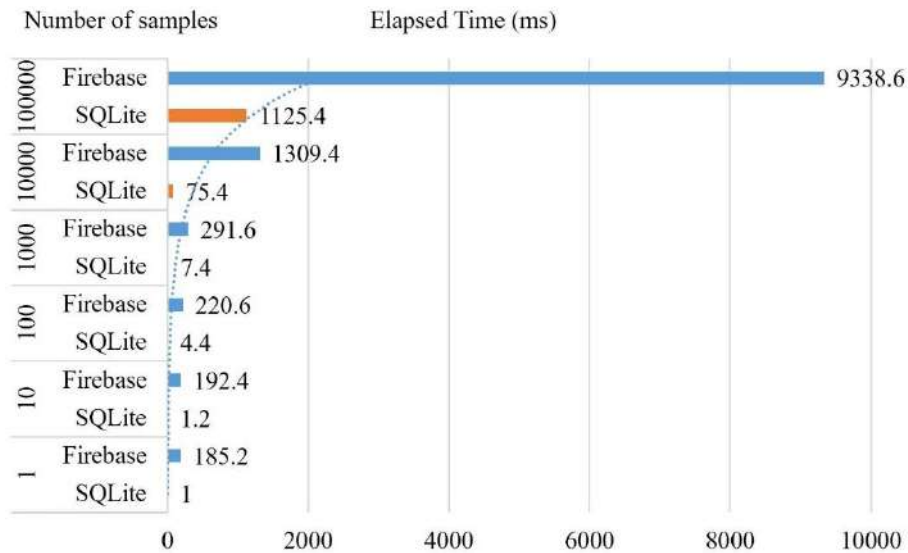
Figure 4. The experimental result of fetching different numbers of data from SQLite and Firebase
