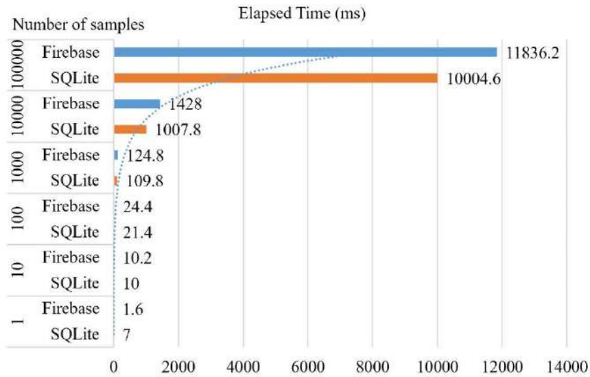
Figure 5. The experimental result of updating different numbers of data in SQLite and Firebase
