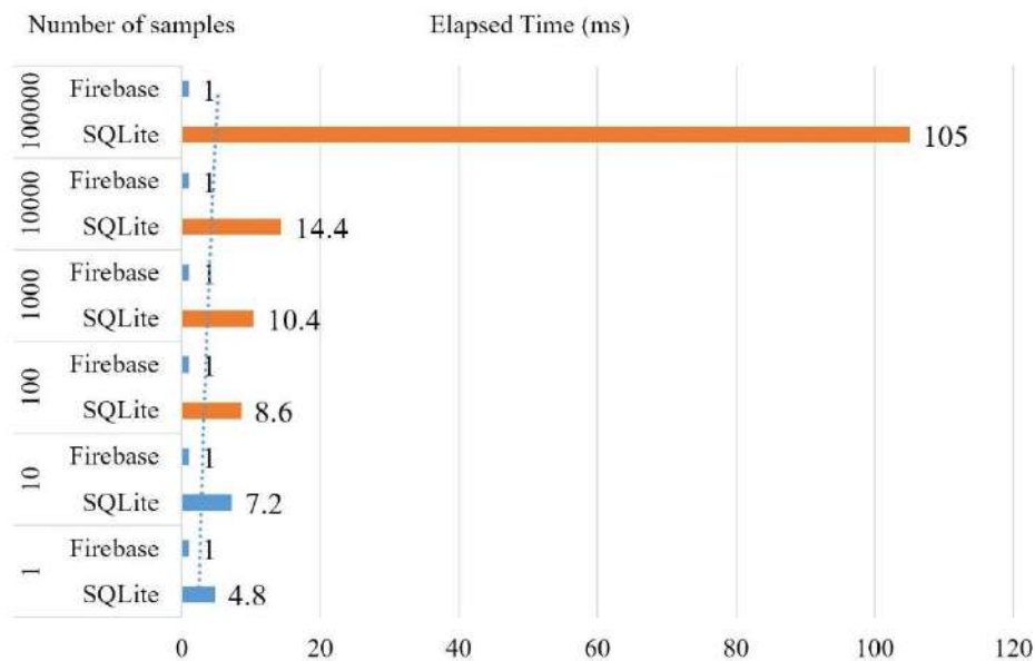
Figure 6. The experimental result of deleting different numbers of data from SQLite and Firebase
